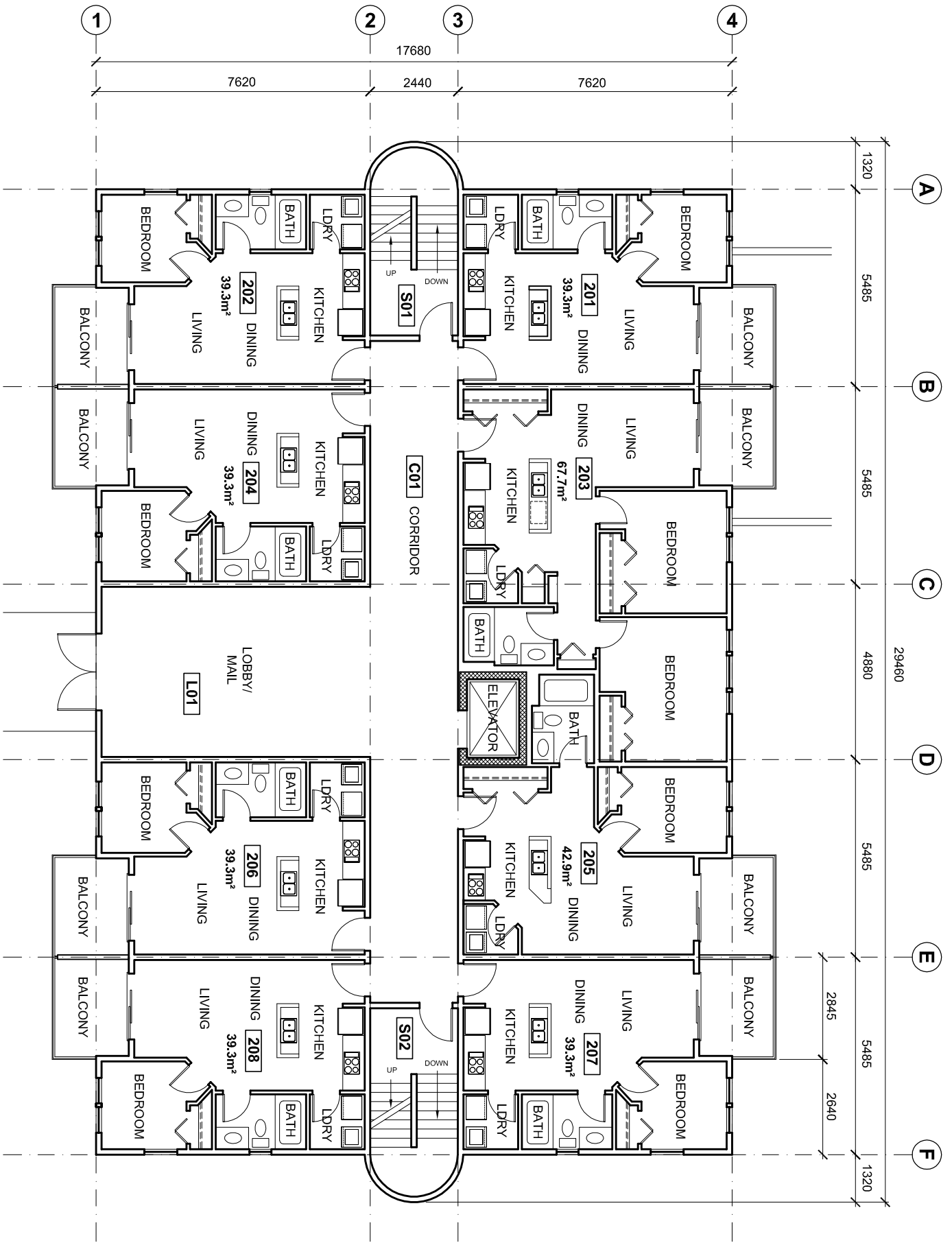
Figure 2: Development Permit Sample Floor Plan
