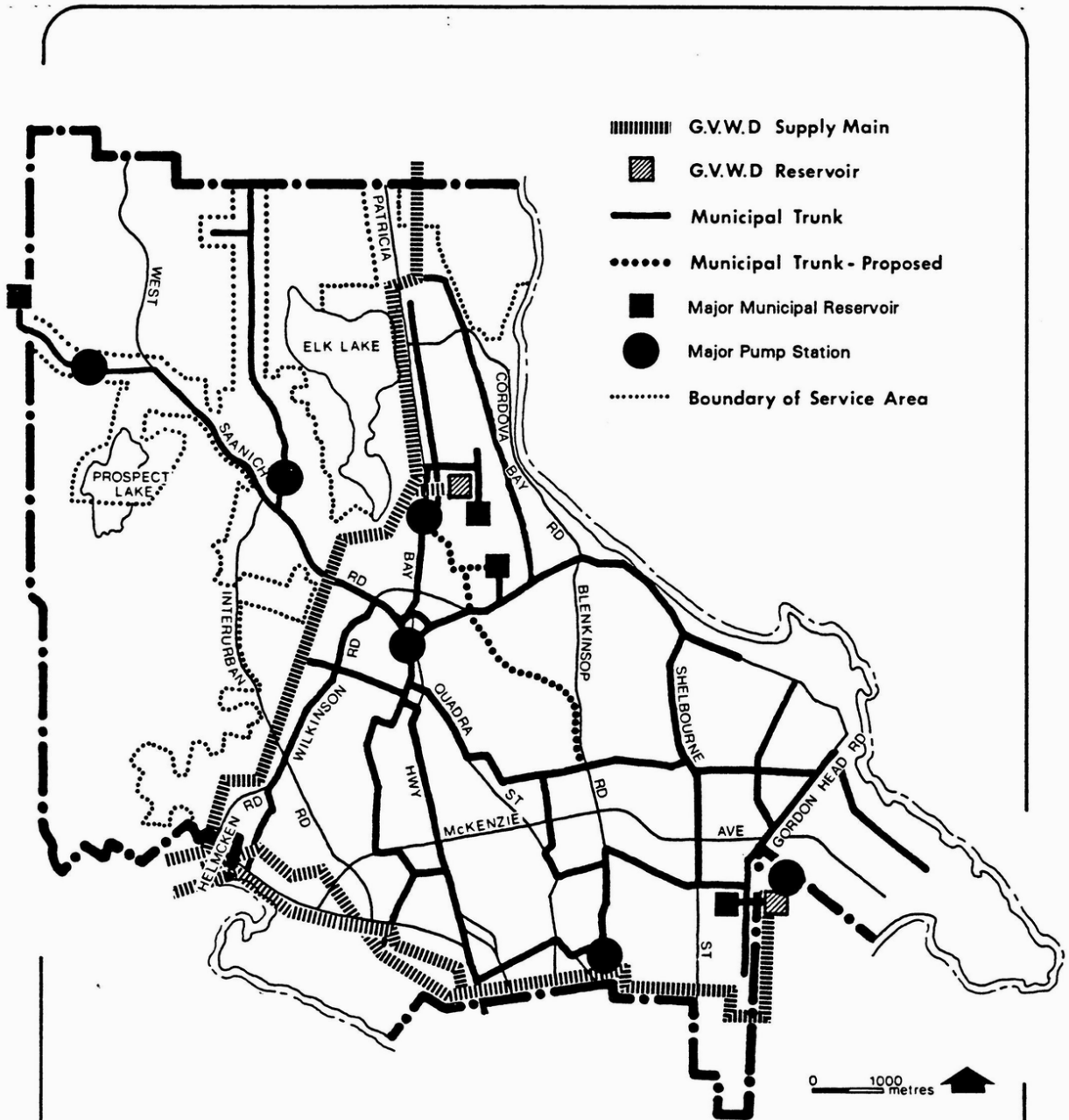
MAP 11.3 WATER DISTRIBUTION SYSTEM
