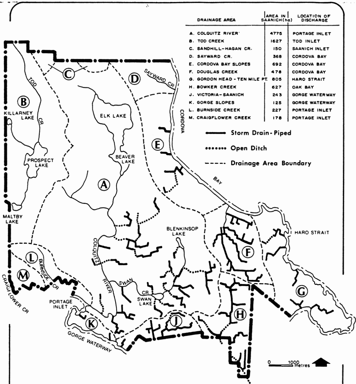
MAP 11.2 STORM DRAINAGE
