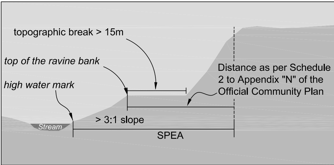
Figure 5: Streamside Protection and Enhancement Area (SPEA) determination for a stream that is located within a ravine
